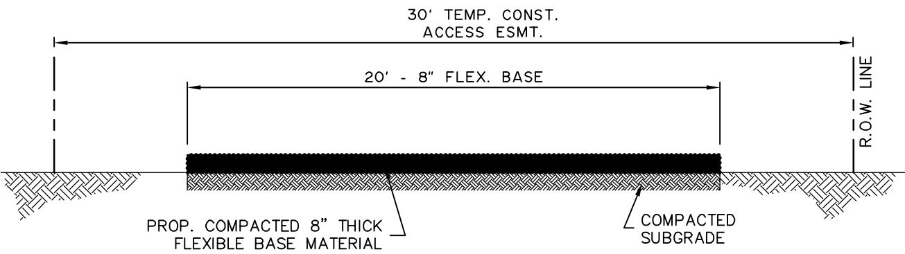
TEMP. CONST. ACCESS EASEMENT DETAIL
