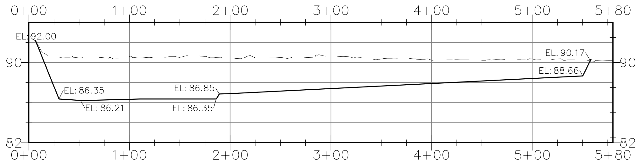
SECTION CC
