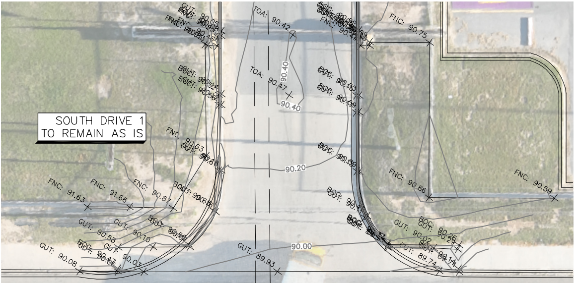
SOUTH DRIVE 1 SCALE: 1"=20'
