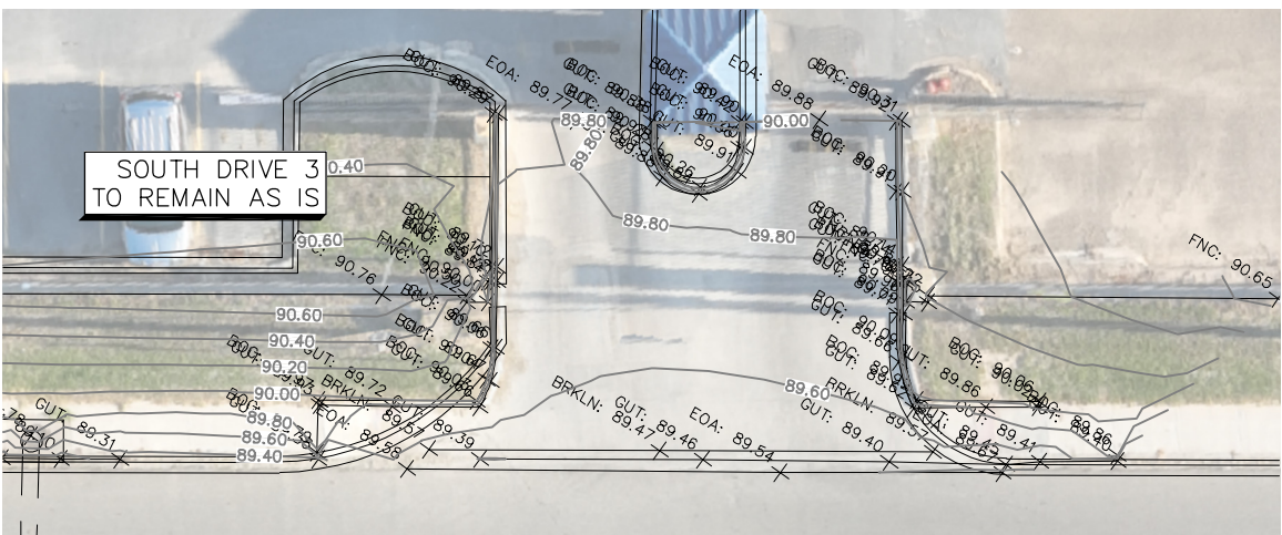
SOUTH DRIVE 3 SCALE: 1"=20'
