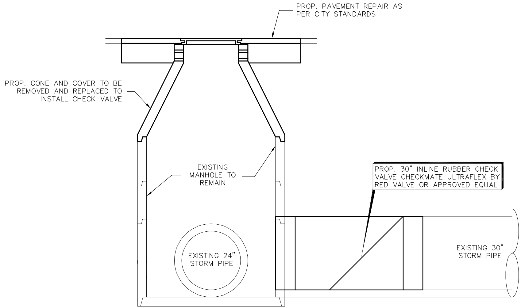
INLINE CHECK VALVE
