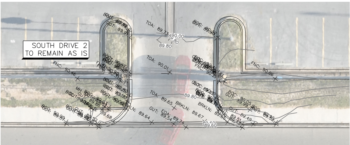
SOUTH DRIVE 2 SCALE: 1"=20'
