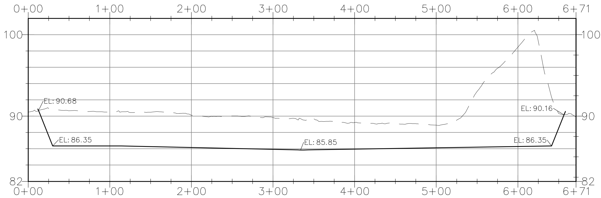
SECTION AA
